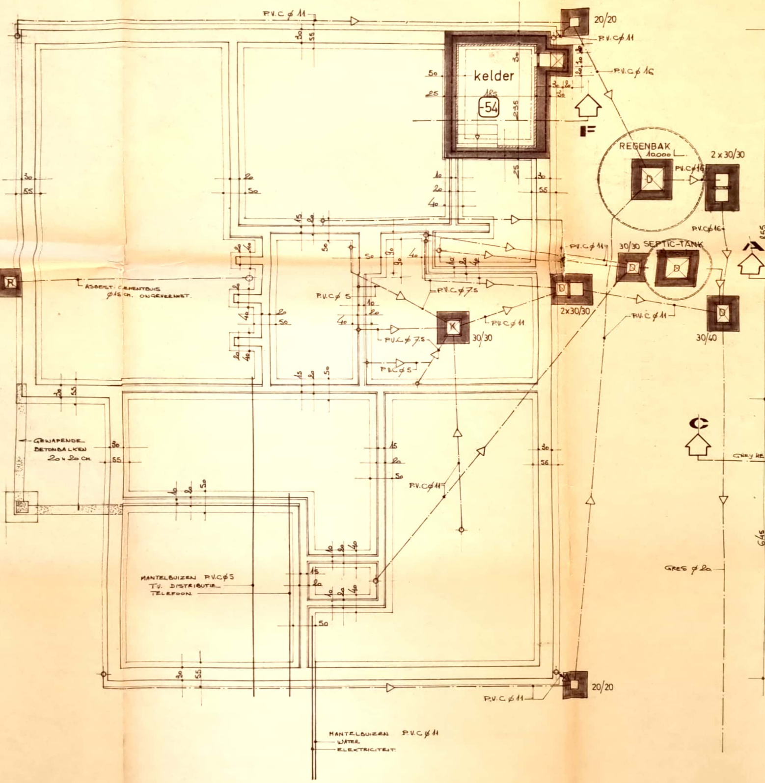
kelder - funderings - rioleringsplan
